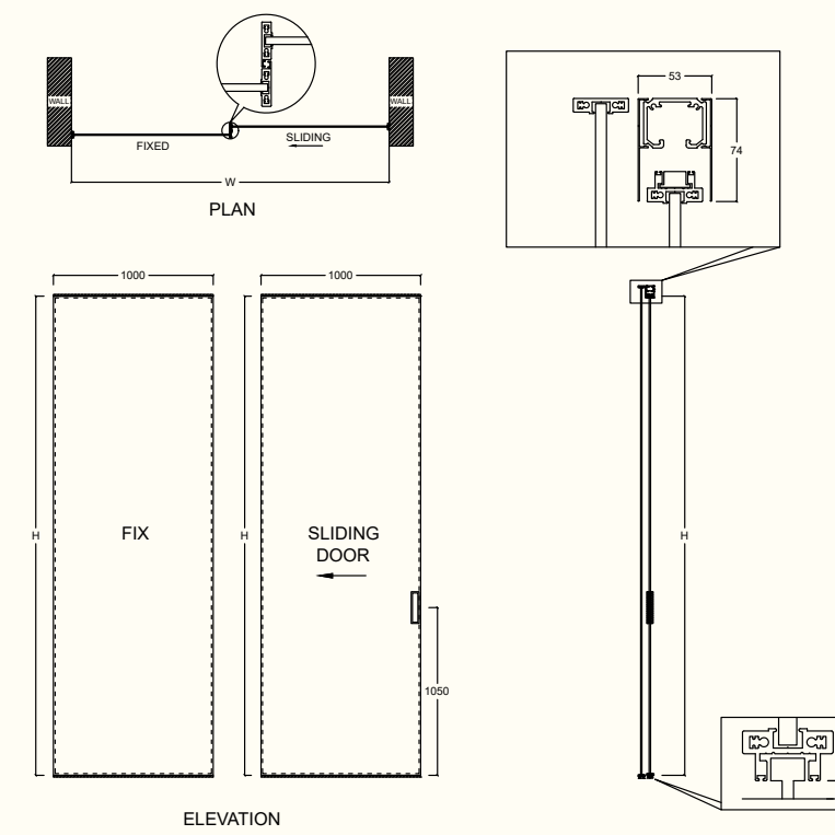
1 FIX + 1 SLIDING SYSTEM
