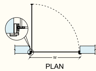
OPENABLE DOOR WITH FRAME
