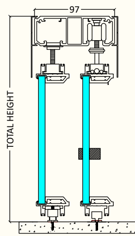
SIDE ELEVATION
