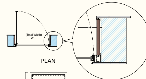
OPENABLE FLUSH DOOR (WITH JAMB)
