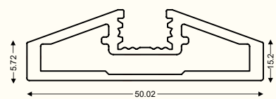
SCP - 311 Side Profile Size : 3 mtr. Finish : Black Matt
