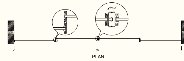
SYNCHRO SLIDING SYSTEM
