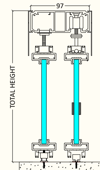
SIDE ELEVATION
