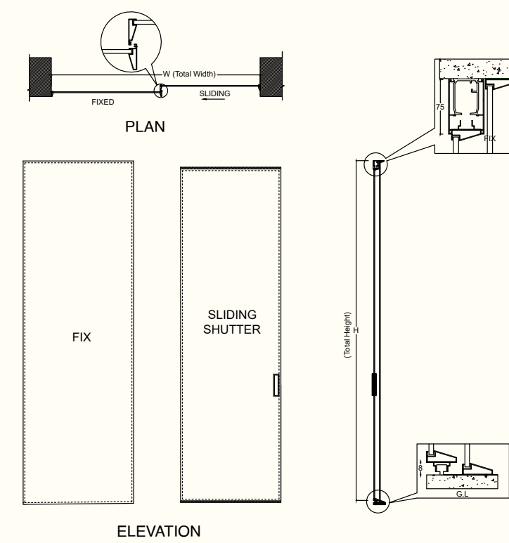
1 FIX + 1 SLIDING SYSTEM
