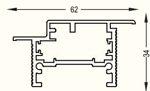
SCP - 201 Aluminium Frame Profile Size : 5.8 mtr. Finish : Black Matt
