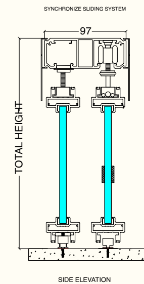
SIDE ELEVATION
