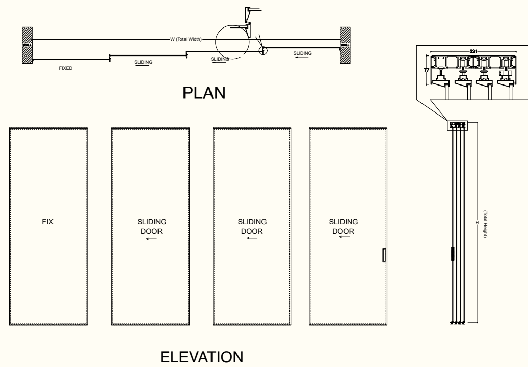
SLIDING TELESCOPIC SYSTEM (1 FIX + 3 SLIDING / 1 FIX + 2 SLIDING / 2 DOOR SLIDING)
