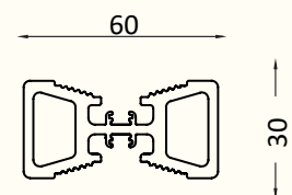
SCP - 301 Column Profile Size : 3 mtr. Finish : Black Matt
