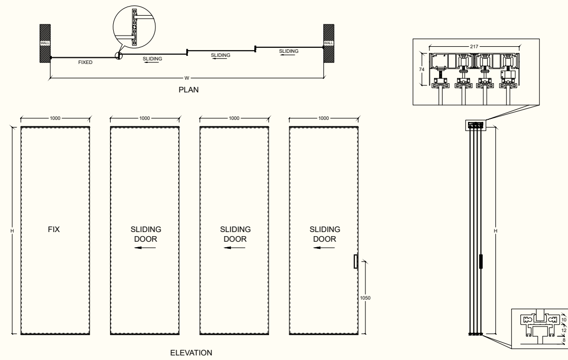
SLIDING TELESCOPIC SYSTEM (1 FIX + 3 SLIDING / 1 FIX + 2 SLIDING / 2 DOOR SLIDING)
