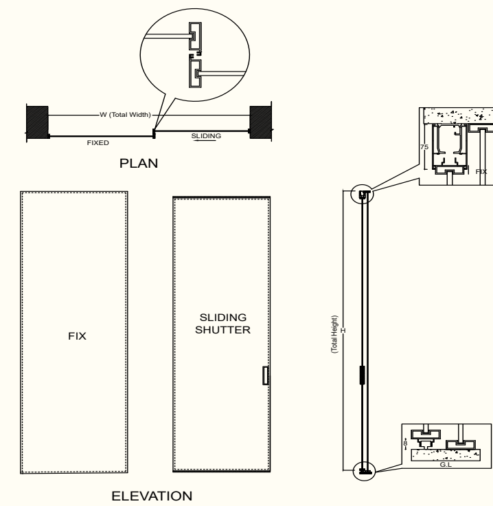
1 FIX + 1 SLIDING SYSTEM
