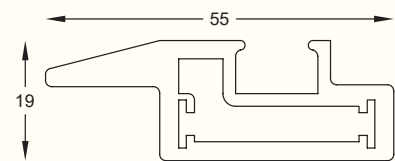
SCP - 171 Frame Profile Size : 5.8 mtr. Finish : Black Matt, Champagne Gold Brush
