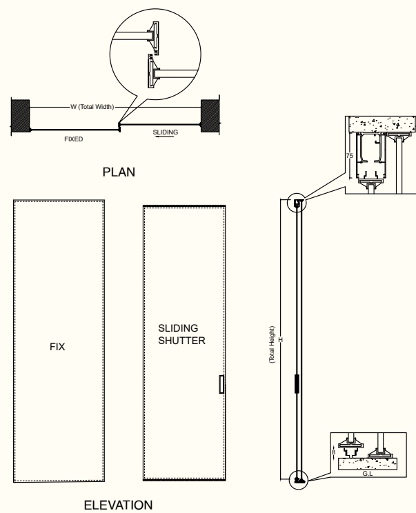
1 FIX + 1 SLIDING SYSTEM
