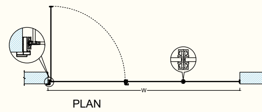
FIX PARTITION WITH OPENABLE DOOR
