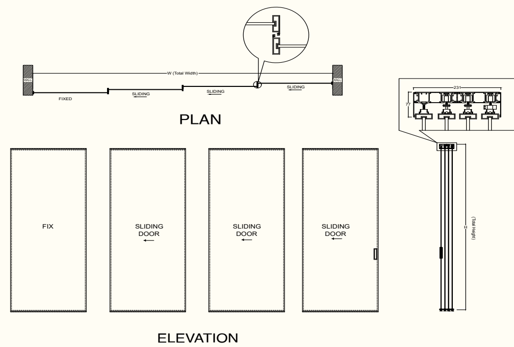
SLIDING TELESCOPIC SYSTEM (1 FIX + 3 SLIDING / 1 FIX + 2 SLIDING / 2 DOOR SLIDING)
