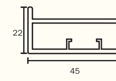
KAPS-31 Frame Profile for 4mm Glass Finish : Alu. Matt, S.S. Brush, Glossy, Black Matt, Rose Gold Grey Matt (Use with KAPS-32)
