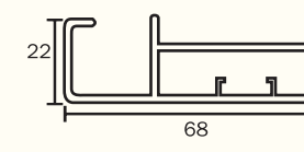
KAPS-32 Frame Profile for 4mm Glass Finish : Alu. Matt, S.S. Brush, Glossy, Black Matt, Rose Gold Grey Matt (Use with KAPS-31)
