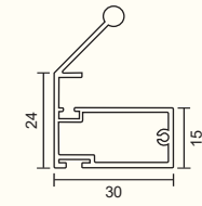
KAPS-54 Frame Profile (5mm to 6mm Glass) Finish : Black Matt
