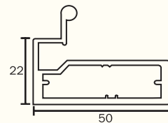
KAPS-09 Frame Profile for 4mm Glass Finish : Alu. Matt, S.S. Brush (Use with KAPS-08)
