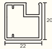
KAPS-02 Frame Profile for 4mm Glass Finish : Alu. Matt, S.S. Brush, Glossy, Black Matt (Use with KAPS-01)
