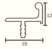
KAPS-33 Handle Profile Finish : Alu. Matt, S.S. Brush, Glossy
