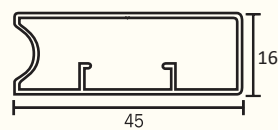
KAPS-43 Frame Profile for 4mm Glass Finish : Alu. Matt, S.S. Brush, Glossy, Black Matt, Rose Gold Grey Matt (Use with KAPS-44)
