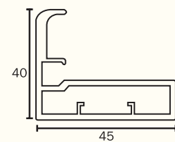
KAPS-16 Frame Profile for 4mm Glass Finish : Alu. Matt, S.S. Brush, Glossy (Use with KAPS-04)
