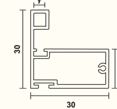
KAPS-53 Frame Profile (5mm to 6mm Glass) Finish : Black Matt
