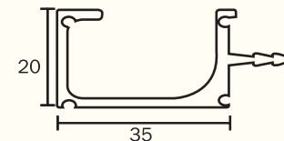
KAPS-29 G-Handle for End Cap Finish : Alu. Matt, S.S. Brush, Glossy, Black Matt
