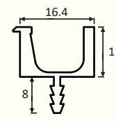
KAPS-30 Aluminium Edge Profile Finish : Alu. Matt, S.S. Brush, Glossy, Black Matt (Use with KAPS-50)
