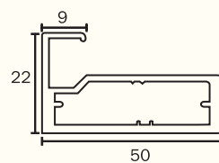
KAPS-17 Frame Profile for 6mm Glass Finish : Alu. Matt, S.S. Brush, Glossy (Use with KAPS-18)
