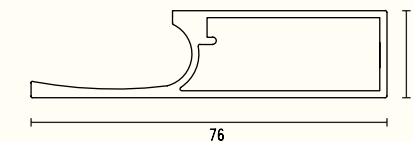
KAPS-58 Handle Profile Finish : Alu. Matt, Black Matt, Rose Gold (Use with KAPS-57)
