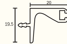
KAPS-41 Handle Profile Finish : Alu. Matt, Black Matt
