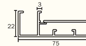
KAPS-24 Frame Profile for 4mm Glass Finish : Alu. Matt, S.S. Brush, Glossy, Grey Matt, Black Matt (Use with KAPS-23)
