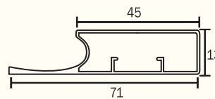
KAPS-44 Frame Profile for 4mm Glass Finish : Alu. Matt, S.S. Brush, Glossy, Black Matt, Rose Gold Grey Matt (Use with KAPS-43)
