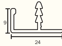
KAPS-35 Edge Profile Finish : Alu. Matt, S.S. Brush, Glossy
