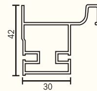
KAPS-46 Vertical Gola Profile Finish : Alu. Matt, S.S. Brush, Glossy, Black Matt
