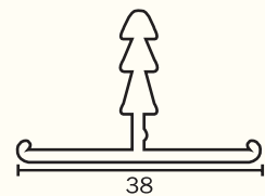
KAPS-14 Edge Profile Finish : Alu. Matt, S.S. Brush, Glossy, Black Matt
