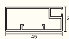
KAPS-22 Frame Profile for 4mm Glass Finish : Alu. Matt, S.S. Brush, Glossy
