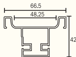
KAPS-47 Vertical Gola Profile Finish : Alu. Matt, S.S. Brush, Glossy, Black Matt
