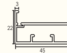
KAPS-23 Frame Profile for 4mm Glass Finish : Alu. Matt, S.S. Brush, Glossy, Grey Matt, Black Matt (Use with KAPS-24)
