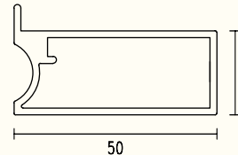
KAPS-55 Frame Profile with Edge Finish : Alu. Matt, S.S. Brush, Black Matt, Rose Gold, Gold Brush, Grey Matt (Use with KAPS-56)
