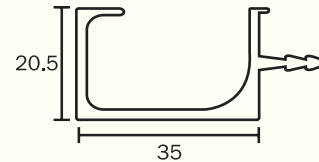
KAPS-06 G Handle Profile Finish : Alu. Matt, S.S. Brush, Glossy, Black Matt, Rose Gold, Grey Matt
