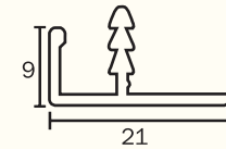
KAPS-21 Edge Profile Finish : Alu. Matt, S.S. Brush, Glossy
