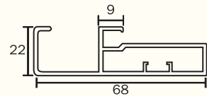
KAPS-05 Frame Profile for 4mm Glass Finish : Alu. Matt, S.S. Brush, Glossy, Black Matt, Rose Gold, Grey Matt, Gold Brush (Use with KAPS-04)
