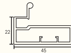
KAPS-45 Frame Profile for 4mm Glass Finish : Alu. Matt, S.S. Brush, Glossy, Black Matt, Rose Gold Grey Matt, Gold Brush (Use with KAPS-04)
