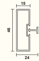
KAPS-52 Frame Profile (5mm to 6mm Glass) Finish : Black Matt
