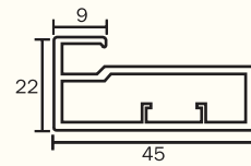
KAPS-04 Frame Profile for 4mm Glass Finish : Alu. Matt, S.S. Brush, Glossy, Black Matt, Rose Gold, Grey Matt, Gold Brush (Use with KAPS-05, 07, 16, 45)
