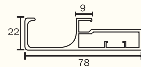
KAPS-07 Frame Profile for 4mm Glass Finish : Alu. Matt, S.S. Brush, Glossy (Use with KAPS-04)
