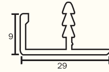
KAPS-36 Edge Profile Finish : Alu. Matt, S.S. Brush, Glossy
