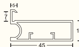
KAPS-59 3mm Edge Frame Profile Finish : Black Matt, Grey Matt, Gold Brush, (Use with KAPS-60)
