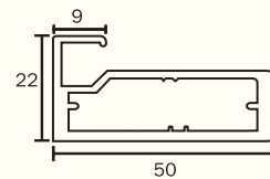
KAPS-08 Frame Profile for 4mm Glass Finish : Alu. Matt, S.S. Brush (Use with KAPS-09)
