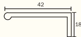
KAPS-10 Handle Profile Finish : Alu. Matt, S.S. Brush, Glossy, Black matt
