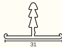
KAPS-13 Edge Profile Finish : Alu. Matt, S.S. Brush, Glossy, Black Matt
