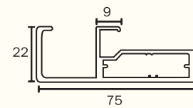
KAPS-18 Frame Profile for 6mm Glass Finish : Alu. Matt, S.S. Brush, Glossy (Use with KAPS-17)
