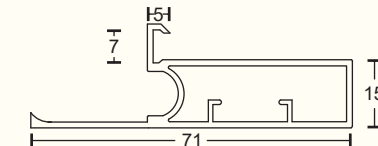
KAPS-60 3mm Edge Handle Profile Finish : Black Matt, Grey Matt, Gold Brush, (Use with KAPS-59)
