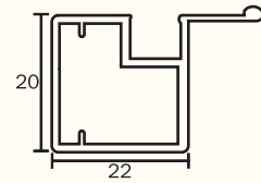
KAPS-01 Frame Profile for 4mm Glass Finish : Alu. Matt, S.S. Brush, Glossy, Black Matt (Use with KAPS-02)
