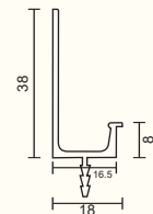
KAPS-50 Handle Profile Finish : Alu. Matt, S.S. Brush, Glossy, Black Matt, Gold Brush (Use with KAPS-30)
