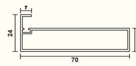
KAPS-51 Frame Profile (5mm to 6mm Glass) Finish : Black Matt
