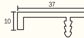
KAPS-42 Handle Profile Finish : Alu. Matt, S.S. Brush, Glossy, Black Matt
