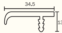
KAPS-03 Handle Profile Finish : Alu. Matt, S.S. Brush, Glossy, Black Matt
