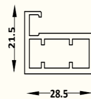
SCP - 28 Top Bottom Profile Size : 3 mtr. Finish : Black Matt, Gold Brush, Grey Matt
