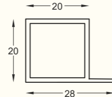
SCP - 07 - 03 Sticking Profile (18mm Product) Size : 3 mtr. Finish : Black Matt
