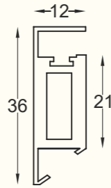
SCP - 08 - 02 Glass Shelf Profile LED Size : 3 mtr. Finish : Black Matt, Gold Brush, Grey Matt
