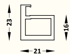
SCP - 06 20mm Square Profile Size : 3 mtr. Finish : Black Matt, Gold Brush, Grey Matt
