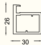
SCP - 31 Frame Profile Size : 3 mtr. Finish : Black Matt, Gold Brush
