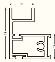
SCP - 24 Handle Profile Size : 3 mtr. Finish : Black Matt, Gold Brush, Grey Matt
