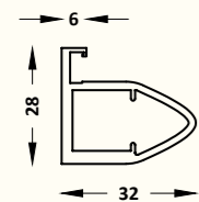
SCP - 03 Oval Shape Profile Size : 3 mtr. Finish : Black Matt, Grey Matt
