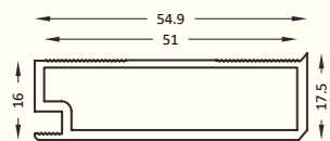
SCP - 14 Side Profile Size : 3 mtr. Finish : Black Matt, Grey Matt
