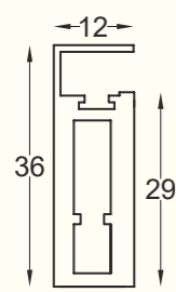
SCP - 08 - 01 Glass Shelf Profile Size : 3 mtr. Finish : Black Matt, Gold Brush, Grey Matt
