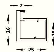
SCP - 04 Square Shape Profile Size : 3 mtr. Finish : Black Matt, Gold Brush, Grey Matt
