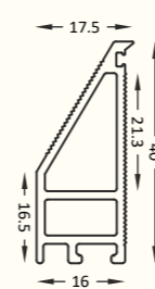
SCP - 18 Handle Profile Size : 3 mtr. Finish : Black Matt, Grey Matt
