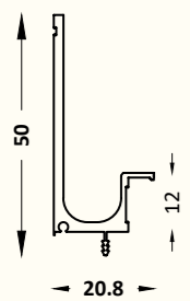
SCP - 19 Alu "J" Edge Profile Handle Size : 3 mtr. Finish : Black Matt
