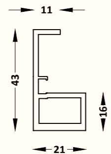
SCPH - 06 - 01 20mm Square Profile Handle Size : 3 mtr. Left/Right (Handle Size : 200mm) Finish : Black Matt, Gold Brush, Grey Matt
