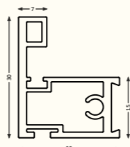
SCP - 23 Handle Profile Size : 3 mtr. Finish : Black Matt, Gold Brush, Grey Matt
