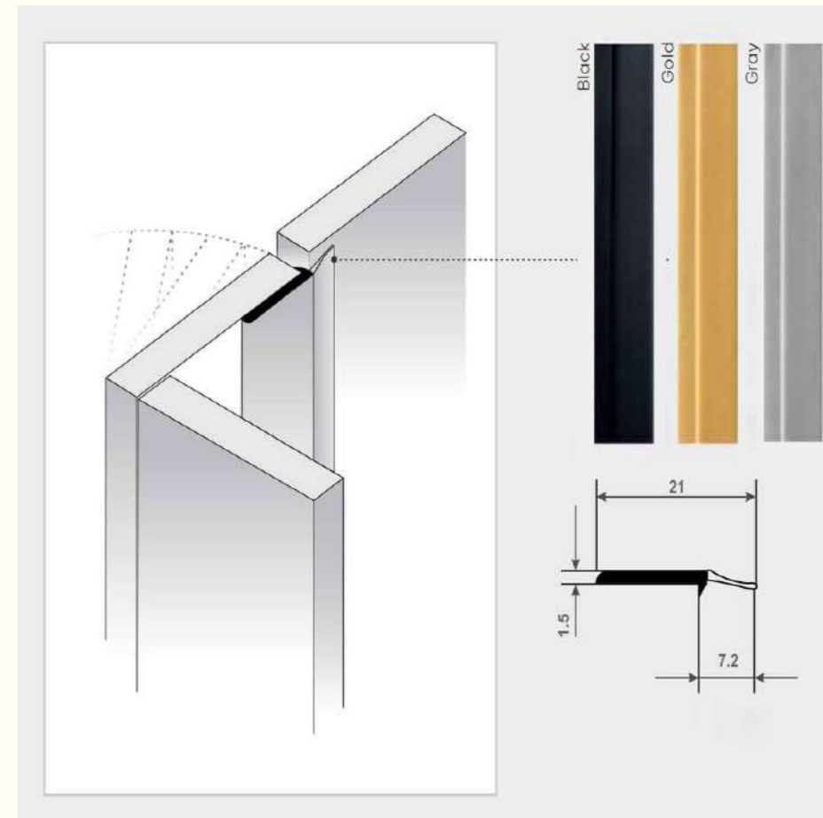
Product Code: SCPA-01 Profile Edge 21mm PVC Door Stripe with adhesive tape of 9mm Finish : Black Matt, Gold Matt, Gray Matt
