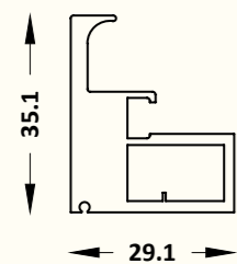
SCP - 26 Handle Profile Size : 3 mtr. Finish : Black Matt, Gold Brush, Grey Matt
