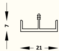
SCP - 05 Wooden Door Profile (For 18mm) Size : 3 mtr. Finish : Black Matt, Gold Brush
