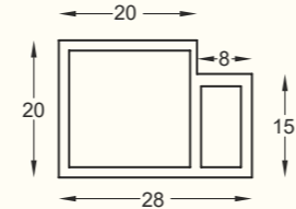
SCP - 07 - 04 Sticking Profile (4mm Product) Size : 3 mtr. Finish : Black Matt
