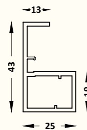
SCPH - 04-01 Square Shape Profile Handle Size : 3 mtr. Left/Right (Handle Size : 200mm) Finish : Black Matt, Gold Brush, Grey Matt
