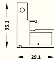
SCP - 27 Side Profile Size : 3 mtr. Finish : Black Matt, Gold Brush, Grey Matt
