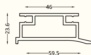
SCP - 92 Shelf Support Profile Size : 3 mtr. Finish : Black Matt
