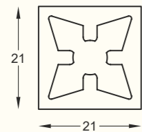
SCP - 07 - 01 Sticking Profile (Vertical) Size : 3 mtr. Finish : Black Matt
