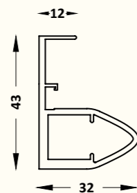
SCPH - 03 Oval Shape Profile Handle Size : 2.7 mtr. (Handle Size : 200mm) Finish : Black Matt, Grey Matt
