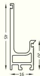
SCP - 17 Handle Profile Size : 3 mtr. Finish : Black Matt, Grey Matt
