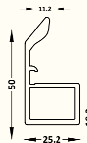
SCPH - 04-04 Slant Square Shape Profile Handle Size : 3 mtr. Left/Right (Handle Size : 1100mm) Finish : Black Matt, Gold Brush, Grey Matt
