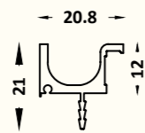
SCP - 20 Alu "C" Edge Profile Handle Size : 3 mtr. Finish : Black Matt
