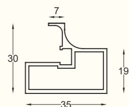
SCP - 01 All Side Handle Profile Size : 3 mtr. Finish : Black Matt, Grey Matt
