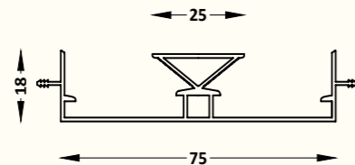
SCPH - 05 Wooden Door Profile Handle Size : 3 mtr. Finish : Black Matt, Gold Brush
