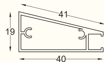
SCP - 02 Slant Profile Size : 3 mtr. Finish : Black Matt, Grey Matt, Gold Brush
