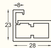
SCP - 13 Pivot Type Top Bottom Profile Size : 3 mtr. Finish : Black Matt, Champagne Gold
