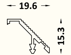
SCP - 29 Alu Cross Edge Profile Size : 3 mtr. Finish : Black Matt
