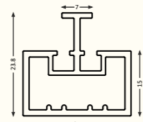
SCP - 22 Divider Profile Size : 3 mtr. Finish : Black Matt, Gold Brush, Grey Matt
